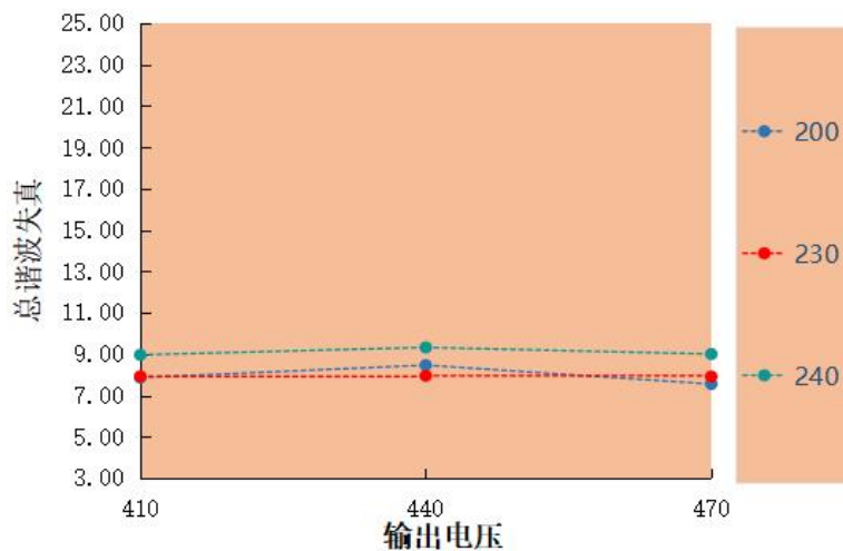
总谐波失真 VS 输出电压 LAS-120H-470A-XP
