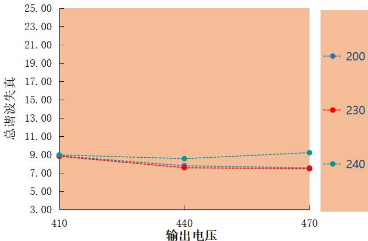
总谐波失真 VS 输出电压 LAS-120H-470A
